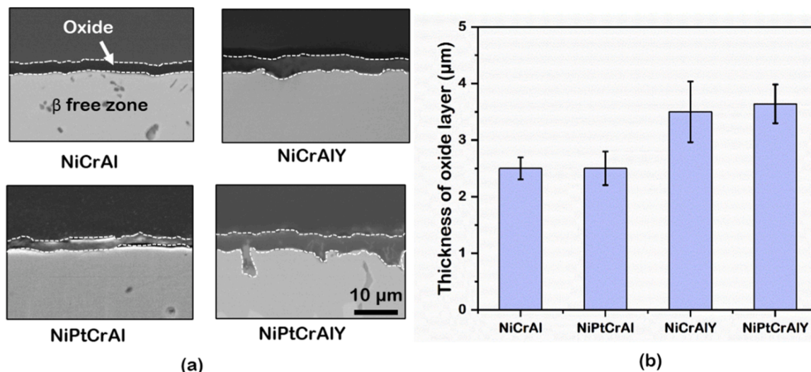
Fig. 4. : Bond coat alloys after oxidation for 100 h at 1100 °C. (a) Cross-sectional micrograph showing the oxide layer (from the un-spalled region) and \beta -free zone, and (b) Plot of oxide layer thickness.
