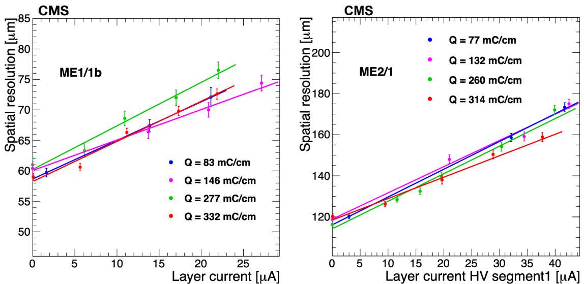
Figure 54. Spatial resolutions for an ME1/1b (left) and ME2/1 (right) chamber using a muon beam while being uniformly illuminated by a 137 Cs photon source to simulate the background from high luminosity pp collisions, as a function of the average current per layer in one HV segment. The results for four different accumulated charges per unit wire length are shown, along with linear fits to each set.
