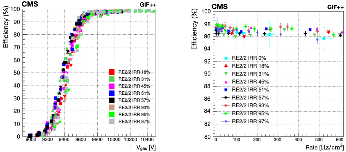
Figure 69. Left: irradiated RE2/2 chamber efficiency as a function of V_{\text{gas}} for different background irradiation rates, up to 600 \text{ Hz}/\text{cm}^2 , and different integrated charge values. Different marker shapes of the same color represent different background rates at the same integrated charge values. Right: irradiated RE2 chamber efficiency at the WP as a function of the background rate at different values of the collected integrated charge. Reprinted from [129], Copyright (2023), with permission from Elsevier.
