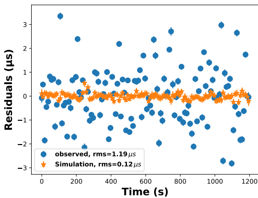
Figure 1. An example of the frequency-averaged timing residuals. The blue circles and orange stars denote the observed residuals obtained from 10 s sub-integrated profiles and residuals obtained with libstempo simulation, respectively (see the beginning of Section 3). The TOAs are obtained from Cycle 41 Band 3 observations for MJD 59545.
