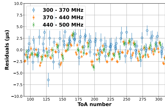
Figure 10. A subset of the ‘Post-fit timing residuals’ of PSR J0437–4715 estimated using 10 second sub-integrated profiles with each having eight frequency channels. The TOAs are subdivided and colour coded as three sets based on the frequency sub-band as shown in the figure. These residuals are plotted serially against the TOA numbers, to check for any potential frequency dependence and its variation for each TOA set in the plotted subset. The complete observation spanned 20 minutes, and only a subset is plotted in this figure for clarity.
