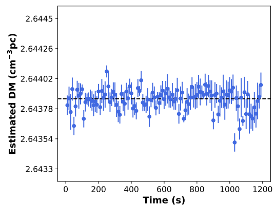
Figure 11. The estimated DM values for each 10 second sub-integration from psrfits to the timing residuals shown in Figure 10. The horizontal dotted line represents the median estimated DM value of 2.64386 \text{cm}^{-3} \text{pc}
