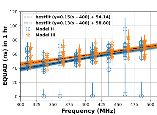
Figure 7. Sub-banded EQUAD scaled to one hour obtained from Model II and III estimation for the sub-bands which had the S/N_{\text{sub}} above the threshold value. The blue circles and orange stars represent the sub-banded EQUAD value of Model II (with EFAC) and III (without EFAC), respectively. The orange stars have been offset by 5 MHz to the right for clarity. The blue and orange shaded lines are from 500 random lines obtained from the posterior distribution of Bayesian regression. The reduced \chi^2 of the best-fit lines are equal to 4.8 for Model II and 1.7 for Model III.
