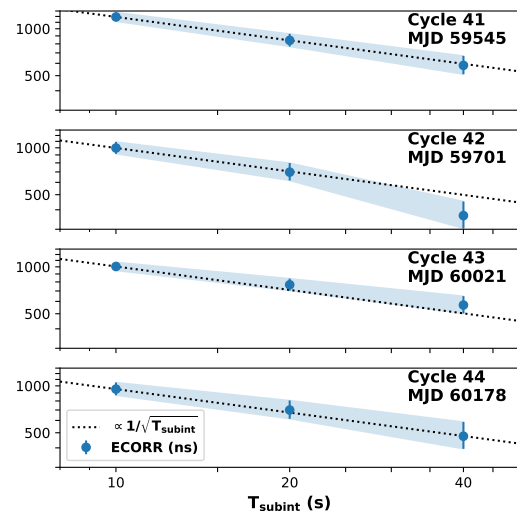
Figure 3. ECORR obtained with different sub-integration. Blue circles denote the ECORR values obtained from different sub-integration times. The black dotted lines shows the fit, which is proportional to the inverse square root of the sub-integration times.
