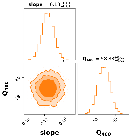
Figure 9. Posterior distributions with 68%, 90%, 99% credible intervals for the parameters fitted using Model III in Figure 7. The point estimates shown above the plots represent the median values and marginalized 68 % credible intervals.
