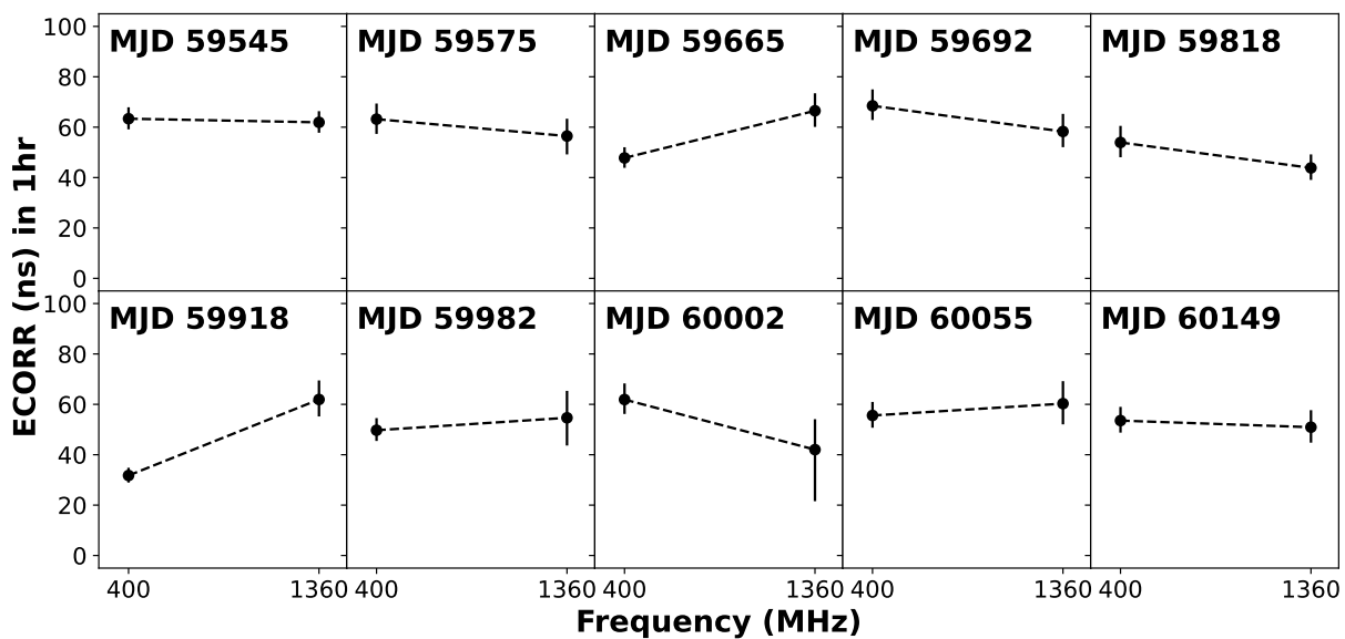
Figure 6. Comparison plots of ECORR for Band 3 and Band 5 for the same epoch obtained from Model I estimation.
