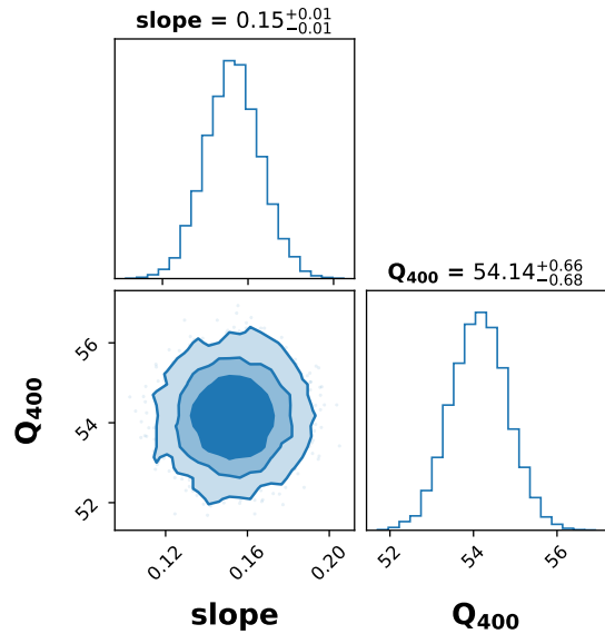
Figure 8. Posterior distributions with 68%, 90%, 99% credible intervals for the parameters fitted using Model II in Figure 7. The point estimates shown above the plots represent the median values and marginalized 68 % credible intervals.
