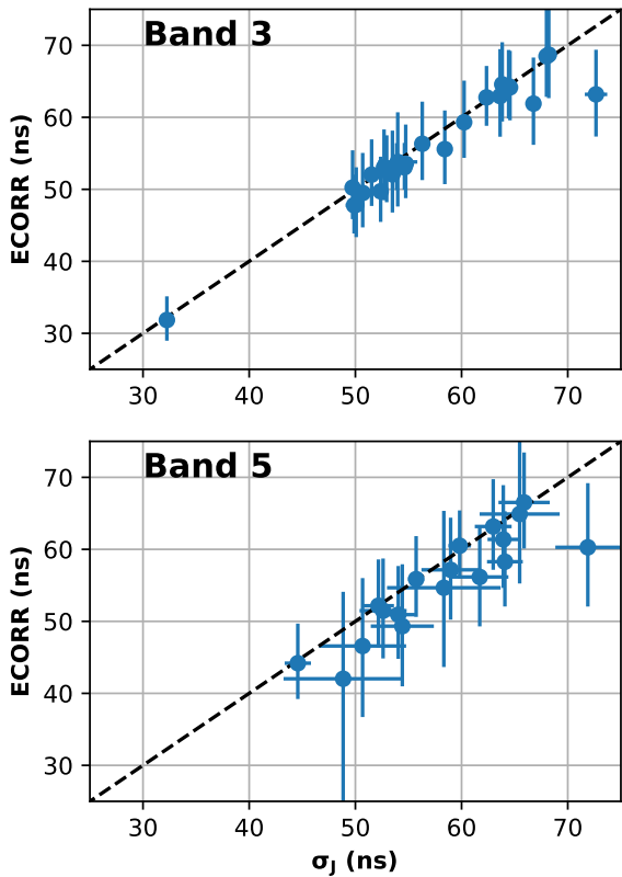
Figure 4. Comparison of jitter amplitudes obtained from Bayesian analysis and traditional method. The blue points denote jitter amplitude. The dashed black line represents the straight line given by y = x . All values are scaled to 1 hour value using equation 2.
