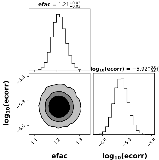
Figure 2. An example of the posterior distribution with 68%, 90%, 99% credible intervals of the Model I parameter estimation. The point estimates shown above the plots represent the median values and marginalized 68% credible intervals. The TOAs are obtained from Cycle 41 Band 3 observations on MJD 59545.
