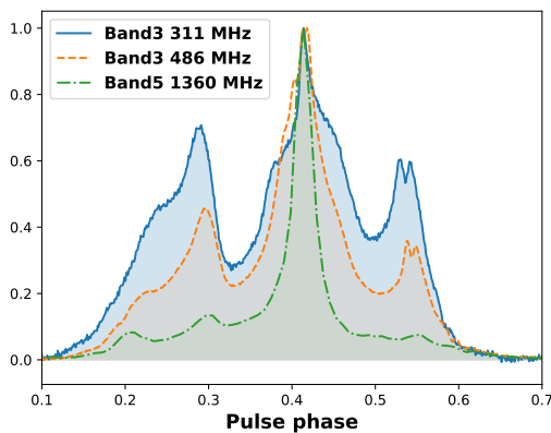
Figure 12. The integrated pulse profile of PSR J0437–4715 at different frequencies. Intensities are normalized. The data used for this plot were obtained from Cycle 41 observation on MJD 59545.
