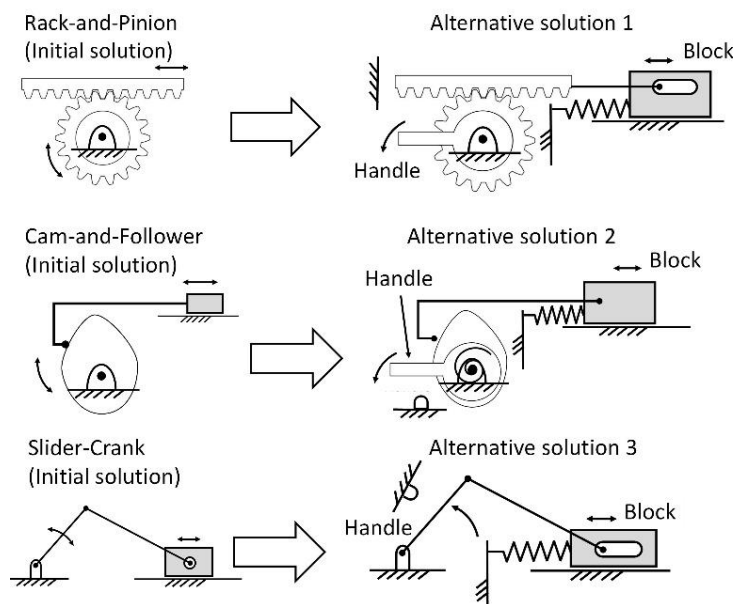
Figure 9. Three alternative solutions are generated with support from the tool for the door-latch design task
