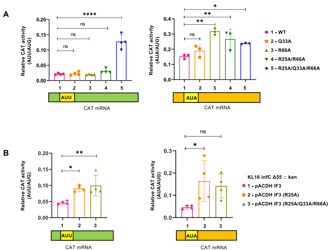
Figure 5. Initiation assays for the non-canonical start codons. (A) CAT assays for AUU start codon (left panel) and AUA start codon (right panel) for different IF3 mutants expressed from the chb locus. (B) CAT assays for AUU start codon (left panel) and AUA start codon (right panel) for different plasmid borne copies of the IF3 mutants in KL16 infC \Delta 55:: kan . Bars represent mean \pm SD for n = 4 . P values, * P < 0.05 ; ** P < 0.01 ; *** P < 0.001 ; **** P < 0.0001 indicate significant differences between samples; 'ns' represent not significant.
