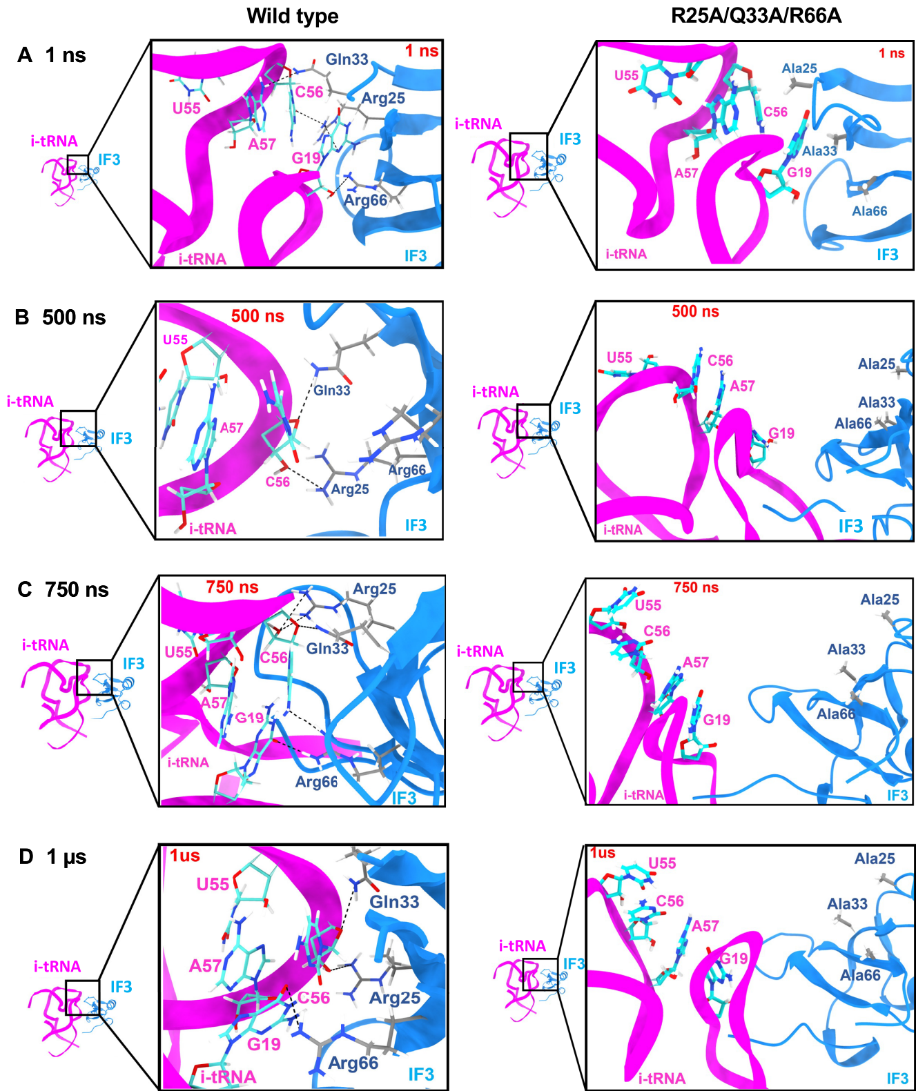
Figure 3. Comparison of the distance between the interacting residues of NTD and i-tRNA between NTD (WT) (left panels) and NTD (R25A/Q33A/R66A) (right panels) during the simulation after 1 ns (A), 500 ns (B), 750 ns (C) and 1 μs (D).
