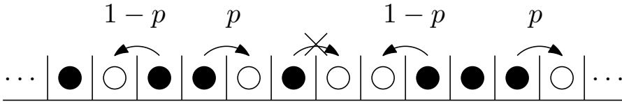
Figure 1: Transitions in the one-dimensional F-TASEP
