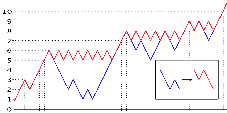
Figure 2: Portion of typical initial (blue, lower) and final (red, upper) height profiles in the F-TASEP; the profile increases monotonically in time from the former to the latter. The vertical dotted lines are at sites in Q . The inset shows the local change in the profile associated with the jump of a single particle, carrying local configuration 1101 to 1011.
