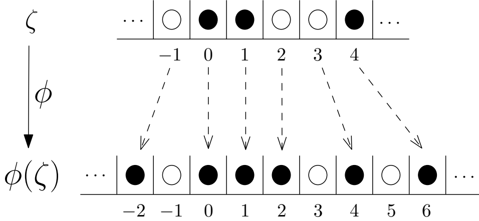
Figure 4: Portion of a typical configuration \zeta , with \zeta(-1:4) = 011001 , and its image under \phi . The dashed arrows show how \gamma_\zeta maps the sites for Y : \gamma_\zeta(-1) = -2 , etc.
