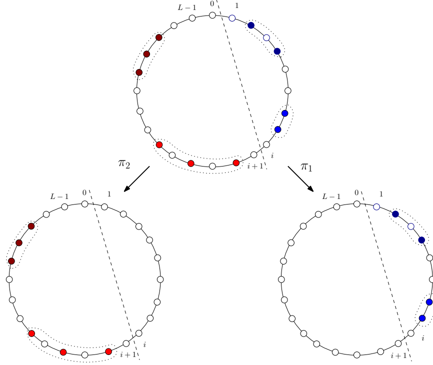
Figure 3: A typical configuration in E_{2,2} (see below) of the finite-volume F-ASEP, with its image under the maps \pi_1 and \pi_2 . The four components are enclosed in dotted loops and are also indicated by color coding.
