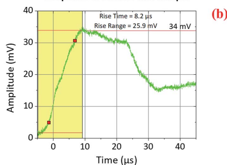
Fig. 7 (a) Measurement of shockwave generated by commercial piezoresistive sensor (b) response of \text{Ti}_3\text{C}_2\text{-MXene} film sample to primary shockwave impact.
