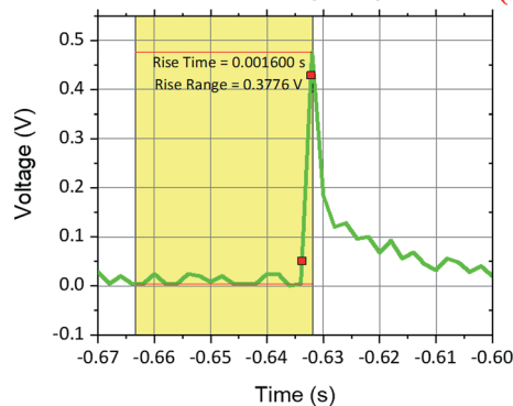
Fig. 8 (a) Variation of response time due to impact forces with changing ball weight (b) response of \text{Ti}_3\text{C}_2\text{-MXene} film sample for ball drop impact (test set-up 3).
