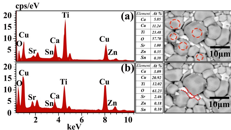
Fig. 4 EDS spectra obtained at selected (a) grains and (b) grain boundary regions for SZS1 ceramics. The marked regions in SEM images correspond to above investigated areas for recording EDS spectra. Their respective relative abundance of elements present is also listed as atomic percentage (At%).
