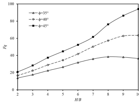
Fig. 8. Variation of breakout factor with embedment ratio.
