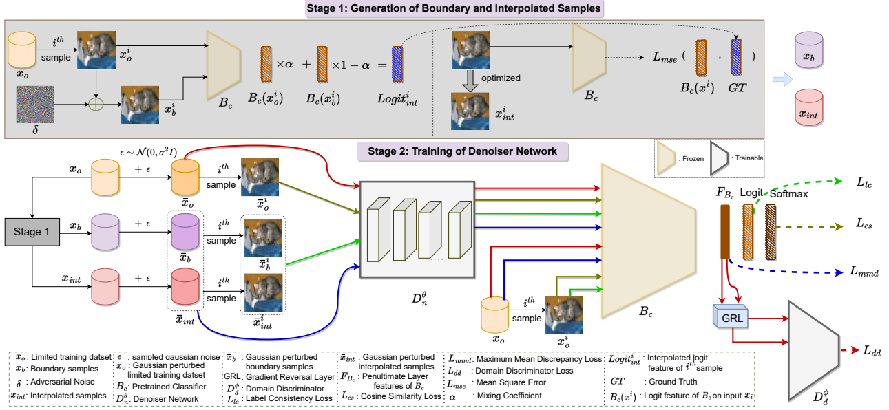
Figure 3. Different stages involved in the proposed method (DE-CROP) that provides robustness guarantees on pretrained classifier ( B_c ) against l_2 perturbations using only limited training samples ( x_o ). Samples crafted via adversarial attack act as proxy boundary samples ( x_b ). Using x_o and x_b , interpolated samples ( x_{int} ) are generated in stage 1. The generated samples along with limited training data are used in stage 2 to train the denoiser network ( D_n^\theta ) by aligning the feature representation at instance and distribution levels using L_{lce} , L_{cs} , L_{mmd} and L_{dd} losses. The forward pass to compute these losses are shown by different colors.
