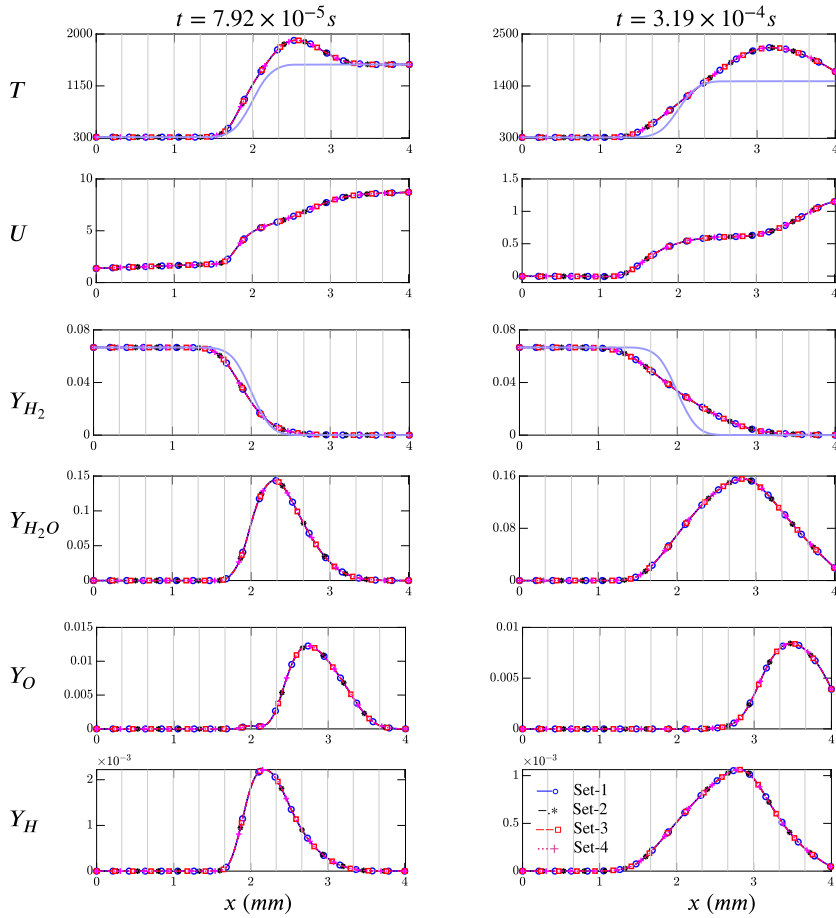
Fig. 13. Asynchrony-tolerant (AT): Instantaneous profiles and error in temperature ( K ), velocity ( ms^{-1} ) and mass fractions of H_2 , H_2O , O and H for non-premixed ignition of H_2 . The different lines: blue (Set-1: p = [0.8, 0.1, 0.1] ), black (Set-2: p = [0.6, 0.3, 0.1] ), red (Set-3: p = [0.4, 0.5, 0.1] ) and magenta (Set-4: p = [1.0, 0.0, 0.0] ) are defined in Table 3. The light blue line indicates the initial condition and the gray vertical lines represent processor boundaries.
