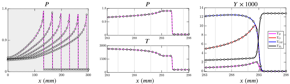
Fig. 14. Asynchrony-tolerant (AT): Pressure (atm) profiles (left) at different times, structure of detonation wave (middle) for pressure (atm) and temperature ( K ) and mass fractions of H , O , OH , H_2 (right). The solid lines are standard WENO and black-dashed line with black symbols (Set-3 in Table 3) corresponds to AT-WENO. Gray vertical lines represent processor boundaries.
