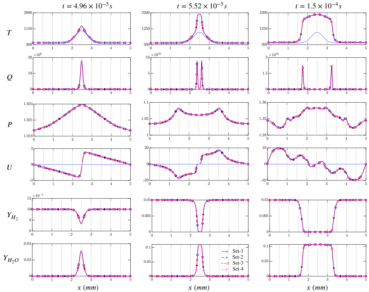
Fig. 7. Asynchrony-tolerant (AT): auto-ignition of a premixed H_2 /air mixture: instantaneous profiles of temperature ( K ), heat-release rate ( Jm^{-3}s^{-3} ), pressure ( atm ), velocity ( ms^{-1} ), and mass fractions of Y_{H_2} and Y_{H_2O} . The different lines: blue (Set-1: p = [0.8, 0.1, 0.1] ), black (Set-2: p = [0.6, 0.3, 0.1] ), red (Set-3: p = [0.4, 0.5, 0.1] ) and magenta (Set-4: p = [1.0, 0.0, 0.0] ) are defined in Table 3. The light blue line indicates the initial condition and the gray vertical lines represent processor boundaries.
