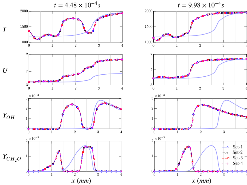
Fig. 10. Asynchrony-tolerant (AT): instantaneous profiles of temperature ( K ), velocity ( ms^{-1} ), and mass fractions of OH and CH_2O radicals for auto-ignition of premixed C_2H_4/air mixtures with temperature fluctuations at the inflow. The different lines: blue (Set-1: p = [0.8, 0.1, 0.1] ), black (Set-2: p = [0.6, 0.3, 0.1] ), red (Set-3: p = [0.4, 0.5, 0.1] ) and magenta (Set-4: p = [1.0, 0.0, 0.0] ) are defined in Table 3. The light blue line indicates the initial condition and gray vertical lines represent processor boundaries.
