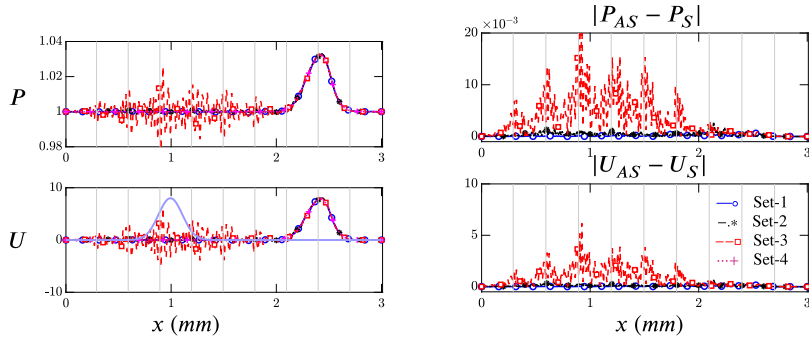
Fig. 4. AS-SFD: instantaneous profiles and errors in pressure ( atm ) and velocity ( \text{ms}^{-1} ) at t = 4 \times 10^{-6}\text{s} . The different lines: blue (Set-1: p = [0.8, 0.1, 0.1] ), black (Set-2: p = [0.6, 0.3, 0.1] ), red (Set-3: p = [0.4, 0.5, 0.1] ) and magenta (Set-4: p = [1.0, 0.0, 0.0] ) are defined in Table 3. The light blue line indicates the initial condition and gray vertical lines represent processor boundaries. AS: Asynchronous with standard finite-difference schemes, S: synchronous.
