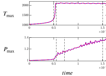
Fig. 6. Temporal evolution of the peak temperature ( K ) and pressure ( atm ) during auto-ignition of a premixture of hydrogen/air in a periodic domain. The different lines (without symbols): blue (Set-1: p = [0.8, 0.1, 0.1] ), black (Set-2: p = [0.6, 0.3, 0.1] ), red (Set-3: p = [0.4, 0.5, 0.1] ) and magenta (Set-4: p = [1.0, 0.0, 0.0] ) are defined in Table 3. The dashed line indicates the time at which the instantaneous scalar and velocity profiles and errors are listed in Table 6 and Table 7.
