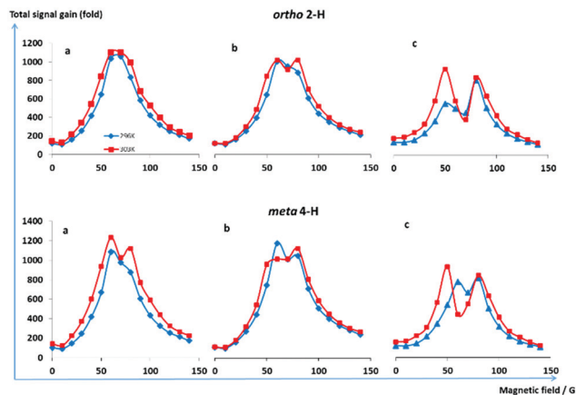
Fig. 2 (a) The SABRE intensity ^1\text{H} NMR signal gains for \text{d}_2\text{-NA} ( \text{d}_2\text{-4,6-nicotinamide} , upper ortho proton and lower meta ) at the indicated temperature as a function of PTF for precatalyst [\text{IrCl}(\text{COD})(\text{Cl-IPhMe}_2)] (5.2 mM) with seven substrate equivalents relative to iridium in \text{d}_4\text{-methanol} solution and 3 bar p\text{-H}_2 . (b) as (a) but with precatalyst [\text{IrCl}(\text{COD})(\text{d}_{16}\text{-Cl-IPhMe}_2)] . (c) as for (a) but in the presence of additional \text{CH}_3\text{CN} .
