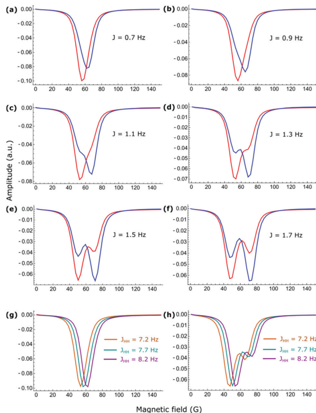
Fig. 1 (a–f) Theoretically predicted ^1\text{H} NMR SABRE signal gain profiles as a function of polarisation transfer field (PTF) for the substrate \mathbf{d}_2 -4,6-nicotinamide. The six plots detailing the ortho (red, H2) and meta (blue, H5) proton responses were produced by the action of a type A catalyst of Scheme 1 and involve the use of the listed interproton couplings between H2 and H5. The hydride–hydride coupling was set to 7.7 Hz, and the trans -hydride–H2 coupling 0.7 Hz. Plot (g) illustrate the effect the hydride–hydride couplings (indicated) on the PTF profile for the ortho proton (H2) resonance when the hydride–H2 coupling is fixed at 0.7 Hz and the H2–H5 coupling fixed at 0.7 Hz. Plot (h) is the same as (g) except now the H2–H5 coupling is 1.5 Hz. See Fig. S10 and S11, ESI† for analogous plots for type B systems.
