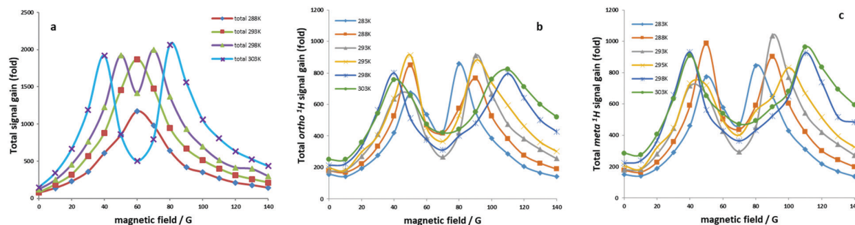
Fig. 3 (a) Summed SABRE intensity ^1\text{H} NMR signal gains for \text{d}_2\text{-4,6-nicotinate} ( \text{d}_2\text{-MN} ) at the indicated temperatures as a function of PTF for precatalyst [\text{IrCl}(\text{COD})(\text{d}_{16}\text{-Cl-IPhMe}_2)] (5.2 mM) with seven substrate equivalents in \text{d}_4\text{-methanol} solution using 3 bar of p\text{-H}_2 . (b) SABRE ^1\text{H} ortho proton NMR signal gain versus PTF for methyl-4,6- \text{d}_2\text{-nicotinate} through the action of [\text{IrCl}(\text{COD})(\text{d}_{22}\text{-IMes})] . (c) as for (b) but the meta proton signal.
