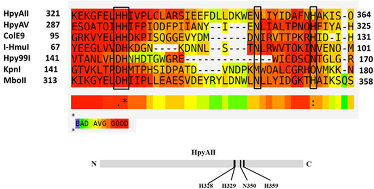
Figure 1. Multiple sequence alignment of HpyAII endonuclease with HHN motif containing enzymes Shading represents the quality of the alignment. Alignment was made using T-COFFEE alignment on EMBnet server. Putative HHN motif residues of HpyAII endonuclease were identified as H328, H329, N350 and H359.
