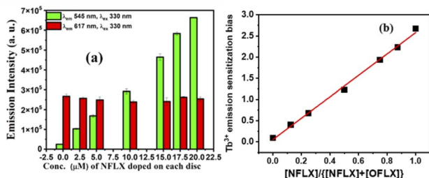
Fig. 6 (a) Tb^{3+} emission at 545 nm and Eu^{3+} emission 617 nm (b) Tb^{3+} sensitization bias in Tb^{3+}/Eu^{3+} /cholate (4.5 mM/0.5 mM/15 mM) gel coated discs with the ratio of NFLX concentration to the total drug concentration in the mixture ( \lambda_{ex} 330 nm).
