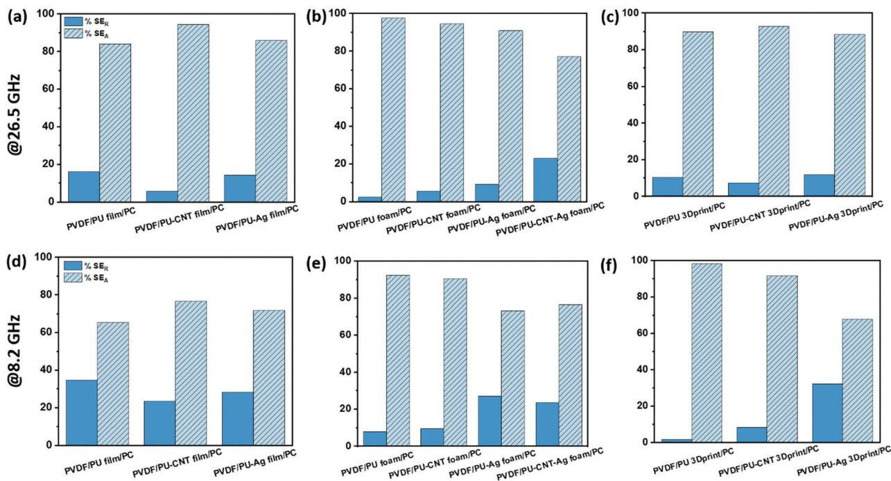
Fig. 14 \% SE_A (light blue bar with stripe pattern) and \% SE_R (dark blue bar with no pattern) at 26.5 and 8.2 GHz: (a and d) with PU-based film as the sandwiched layer in between PVDF–rGO– Fe_3O_4 film and PC–CNT film; (b and e) with PU-based foam as the sandwiched layer in between PVDF–rGO– Fe_3O_4 film and PC–CNT film; (c and f) with PU-based 3D print structure as the sandwiched layer in between PVDF–rGO– Fe_3O_4 film and PC–CNT film.
