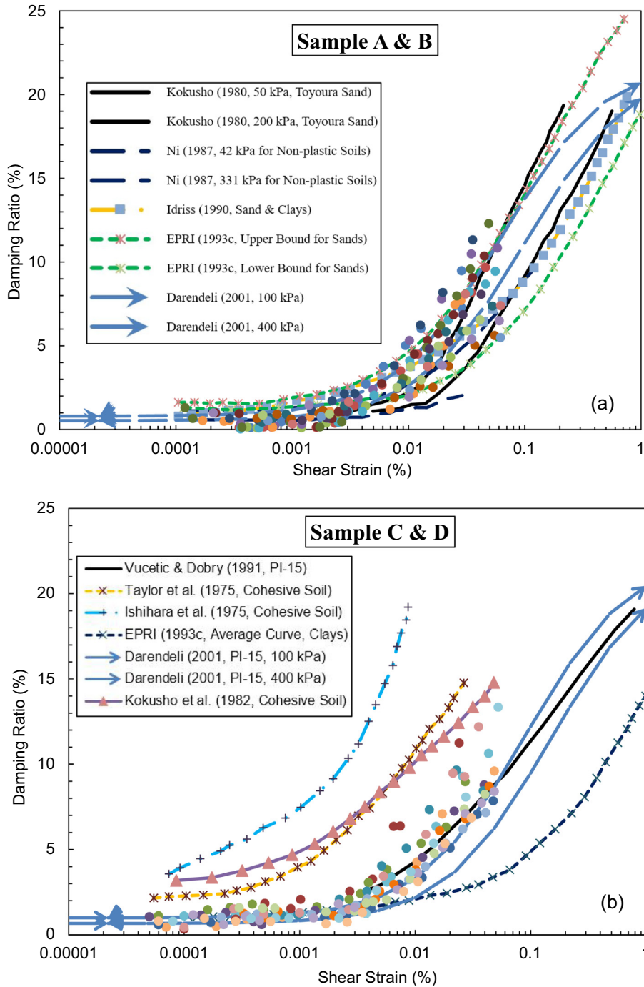
Fig. 11. (a) and (b) Comparison of damping ratio with other investigators for sands and cohesive soils.
