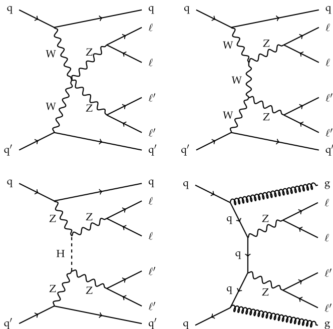
Fig. 1. Representative Feynman diagrams for the EW- (top row and bottom left) and QCD-induced production (bottom right) of the ZZjj \rightarrow \ell\ell\ell'ell'jj ( \ell, \ell' = e or \mu ) final state. The scattering of massive gauge bosons as depicted in the top row is uniterized by the interference with amplitudes that feature the Higgs boson (bottom left).
