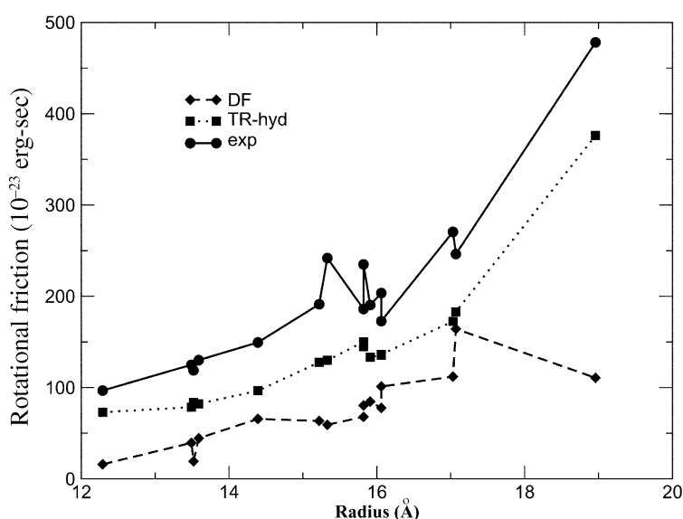
Figure 3. Rotational friction coefficients obtained from the experiment, hydrodynamic and dielectric friction plotted against radius for some proteins.
