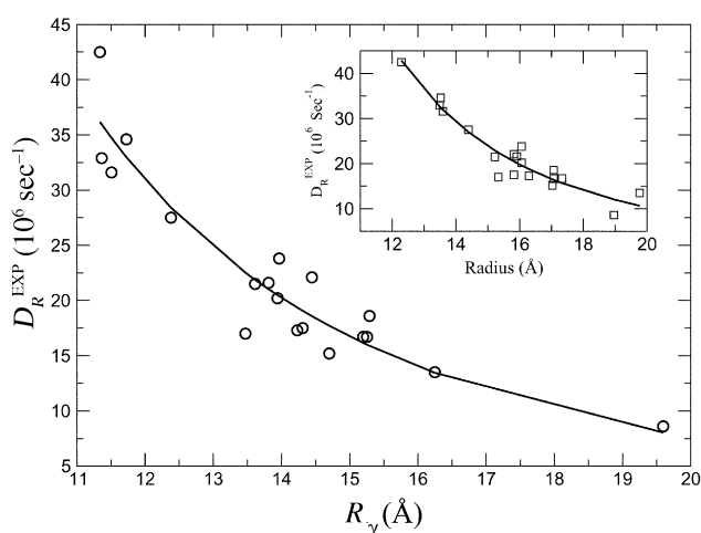
Figure 2. Experimental rotational diffusion ( D_R^{\text{EXP}} ) coefficients are plotted against the calculated R_g for some proteins. Circles show experimental values and solid line is the power law fit with an exponent 2.75. (Inset) Squares show plot of D_R^{\text{EXP}} against radius of the protein obtained from total mass. Solid line is a power-law fit, with an exponent 2.92.
