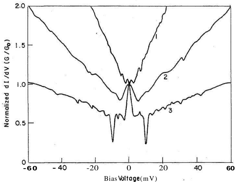
Figure 2. The normalized conductance data ( G/G_0 ) for point contact junctions formed by Au tip on Bi(2212) single crystal with zero bias conductance ( G_0 ) varying by almost three orders in magnitude. The G_0 values: 3.9 \times 10^{-2}\text{ S} for curve 1, 7.5 \times 10^{-4}\text{ S} for curve 2 and 5.5 \times 10^{-2}\text{ S} for curve 3.
