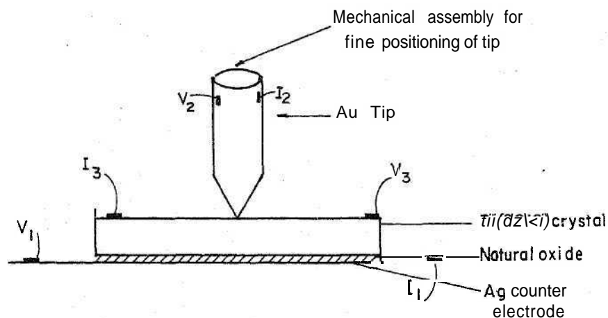
Figure 1. Schematic of the experimental arrangement I 's are current leads and V 's are potential leads. Combination 2-3 is used for the point contact junction and combination 1-3 for the natural oxide planar tunnel junction.
