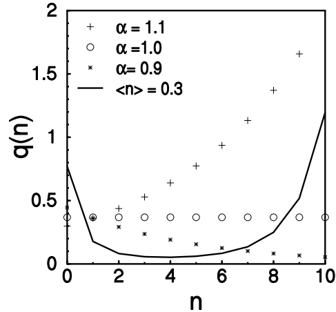
FIG. 2. Generic behaviours of the sequence \{q_n\} for different classical states. First three are coherent states with different displacements and the fourth one is a thermal state.
