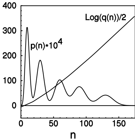
FIG. 1. “Classical” oscillation in the photon number distribution, for an incoherent mixture of coherent states with density matrix \rho = \lambda_1|\alpha_1\rangle\langle\alpha_1| + \lambda_2|\alpha_2\rangle\langle\alpha_2| + \lambda_3|\alpha_3\rangle\langle\alpha_3| + \lambda_4|\alpha_4\rangle\langle\alpha_4| + \lambda_5|\alpha_5\rangle\langle\alpha_5| with |\alpha_1|^2 = 10 , |\alpha_2|^2 = 30 , |\alpha_3|^2 = 60 , |\alpha_4|^2 = 90 , |\alpha_5|^2 = 130 and \lambda_1 = \lambda_2 = 0.25 , \lambda_3 = 0.2 , \lambda_4 = 0.18 , \lambda_5 = 0.12 . The symbols p(n) , q(n) stand, respectively, for p_n , q_n of the text. It may be noted that q_n exhibits no oscillations for this classical state.
