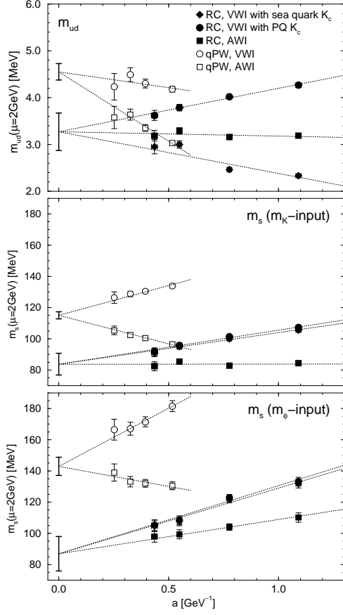
Figure 1: Continuum extrapolations of m_{ud} (top), and m_s with m_K -input (middle) and m_\phi -input (bottom) [5]. Open and filled symbols are results for N_f = 0 and 2.
