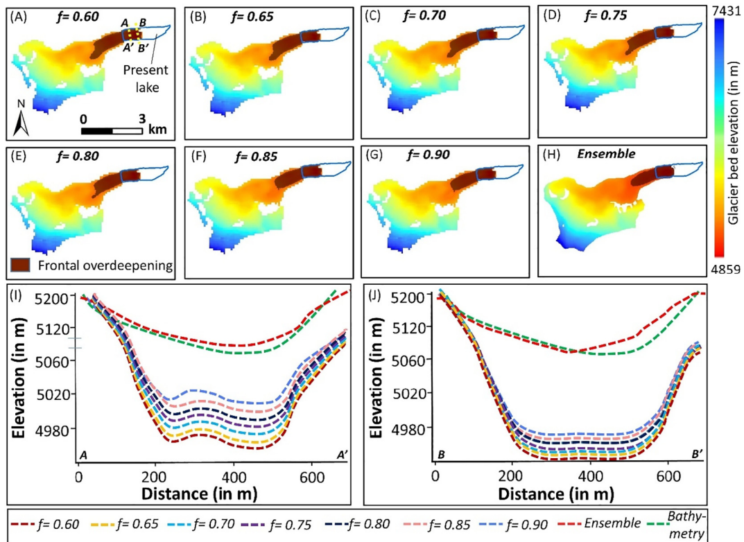
Fig. 4. Spatially distributed modeled glacier bed for different values of 'f' using GlabTop (A-G); Ensemble (H) (Farinotti et al., 2019); (I-J) cross-sectional profiles of glacier beds along AA' and BB'.
