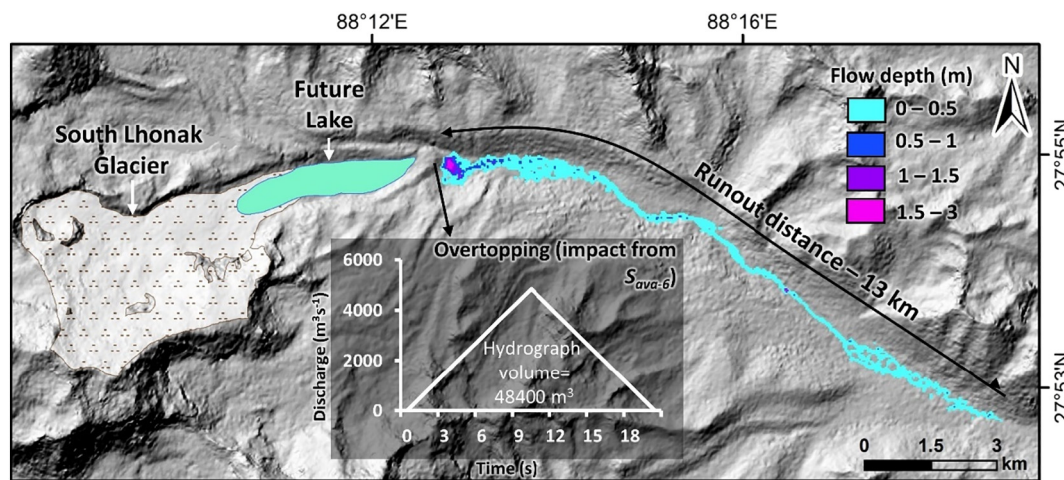
Fig. 8. Overtopping flow depth along the channel resulting from avalanche impact ( S ava-6 ); the subset shows the overtopping hydrograph calculated based on impact wave from S ava-6 ; note that due to relatively flat terrain just in front of the lake, there is a significant loss in the momentum of the flow and the flow tends to slow down and terminates at 13 km downstream of the lake i.e. 33 km upstream of Lachen.
