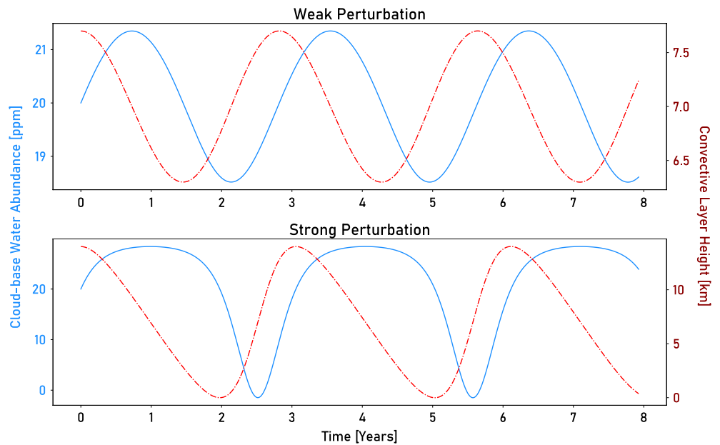
Figure 4. A simple first-order Eulerian scheme integration of the Equations 21 and 22 with [a,b] = 10^{-7}s^{-1} showing interannual oscillations. The integrations were initialized with [x,y] = [0,0.1] for the top panel and [x,y] = [0,1] for the bottom panel. The blue solid line shows the cloud-base water abundance ([H_2O]) , while the red dashed line shows the convective layer height ( L ). In the weak perturbation limit, the oscillations are harmonic and in the strong perturbation limit, they can be described as recharge-discharge oscillations.
