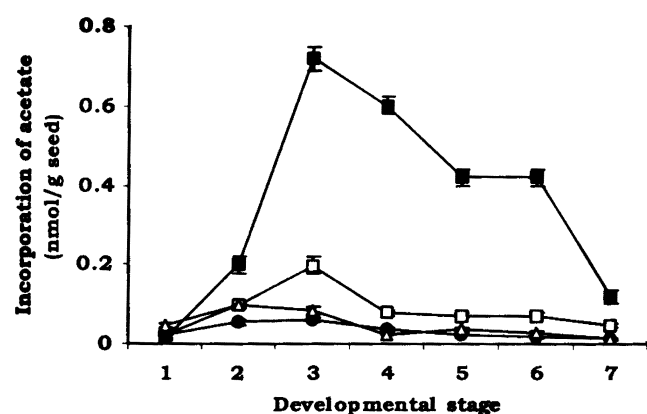
Figure 2. Incorporation of [ ^{14}\text{C} ]acetate into lipids by developing seeds of G. indica . Seed slices (500 mg) from each stage were incubated for 4 h with [ ^{14}\text{C} ]acetate and the radioactivity in TAG (■), DAG (●), PC (□) and PE (△) quantified. Data are expressed as mean \pm SD of three sets of determinations.
