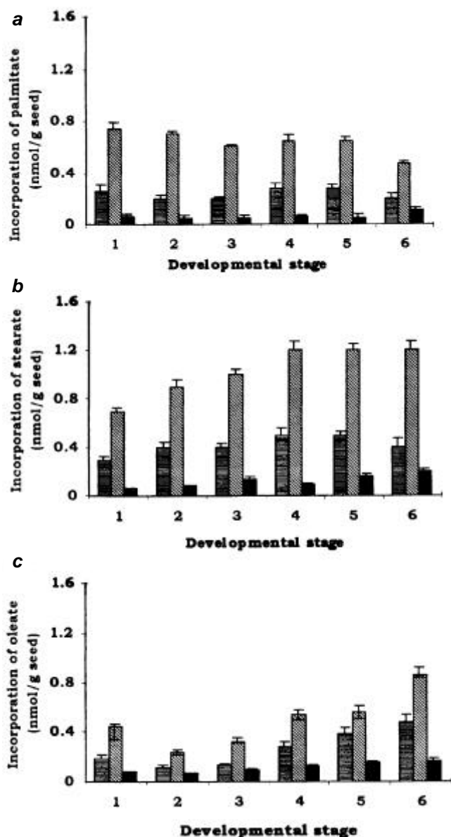
Figure 3. Incorporation of 14 C-labelled fatty acids into lipids by developing seeds of G. indica . Seeds at various developmental stages (500 mg) were incubated with [ 1-14 C]palmitate a , [ 1-14 C]stearate b , and [ 1-14 C]oleate c , for 4 h, and incorporation of radioactivity into TAG (□), DAG (▣) and PC (■) by developing seeds was determined. Values are mean ± SD of three determinations.
