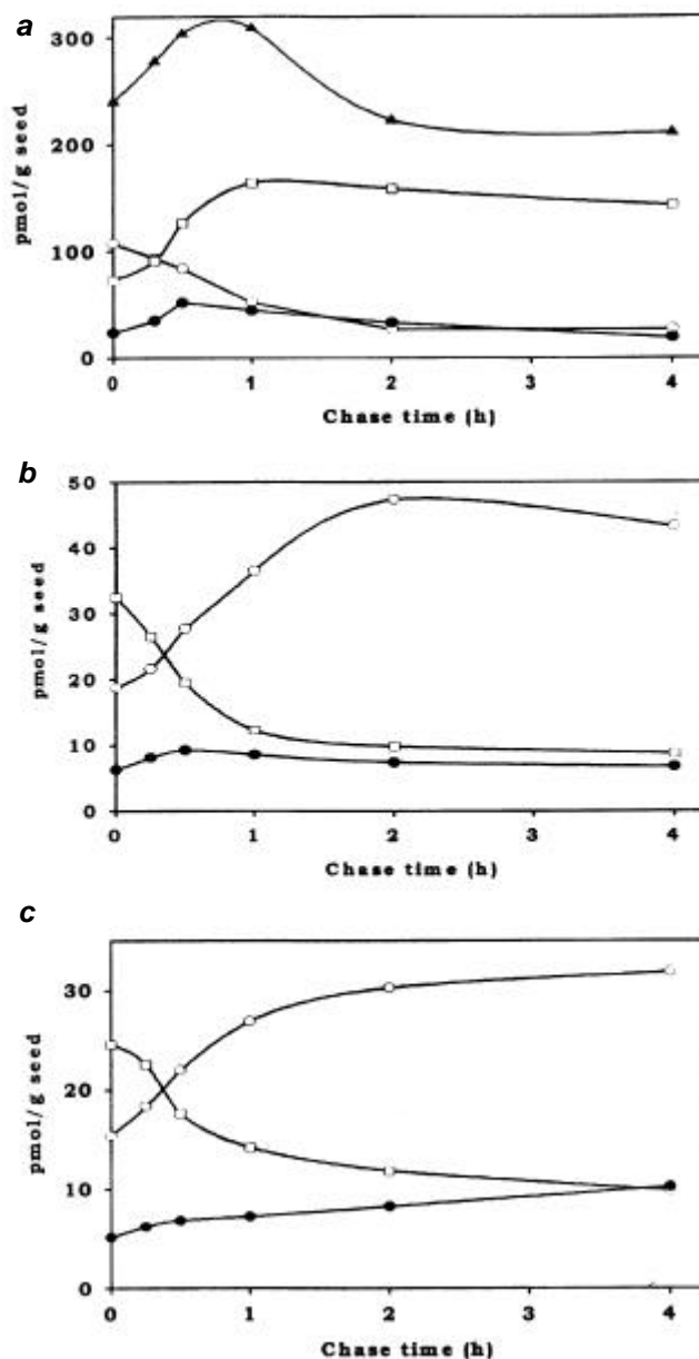
Figure 4. Pulse-chase labelling of G. indica seed lipids with [ 14 C]acetate. Stage-3 immature seeds were pulsed with [ 14 C]acetate for 15 min; after labelling, the tissues were then chased with unlabelled acetate. At different time intervals, total lipids were extracted and analysed in silica-TLC. a , Amount of radioactivity incorporated into total lipids (▲), PC (O), DAG (●) and TAG (□) at indicated time points after the label was removed. b and c , Radiolabelled PC, DAG and TAG from the various chase periods were purified and converted to FAME. The labelled FAMES were resolved on reverse-phase TLC. The proportion of radioactivity in the stearoyl b and oleoyl c moieties of PC (□), DAG (●) and TAG (O) was determined. Values are mean of three separate experiments from the same batch of seeds and each performed in duplicate.
