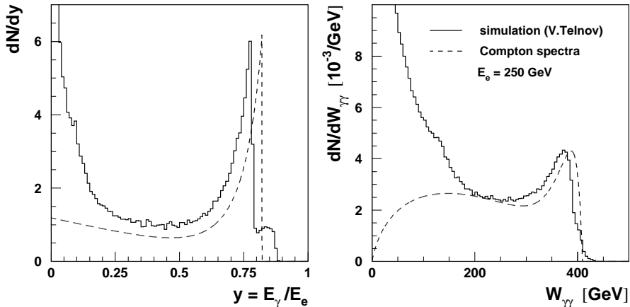
Figure 6: The energy spectrum for the single photon and the spectrum in the two photon invariant mass W_{\gamma\gamma} for the backscattered laser photons after inclusion of the nonlinear effects as parametrised in [12] and compared with simulation [13], for E_{beam} = 250 GeV.
