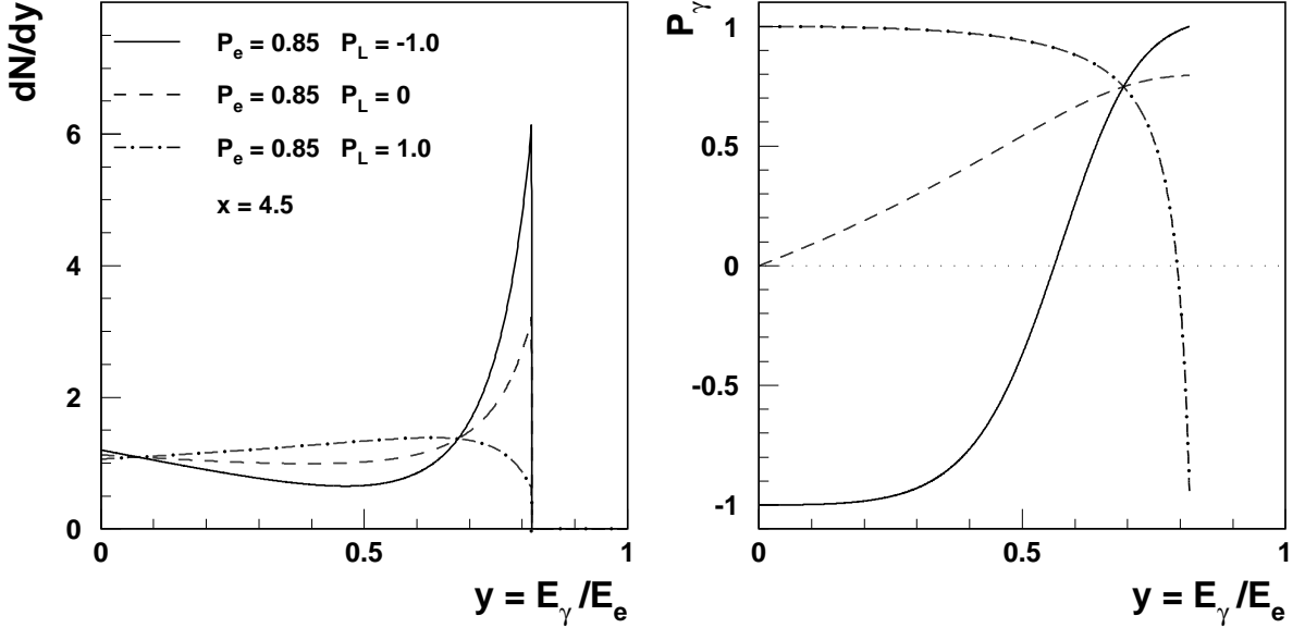
Figure 2: Energy spectrum and the polarisation expected for the backscattered laser for ideal case [11]
