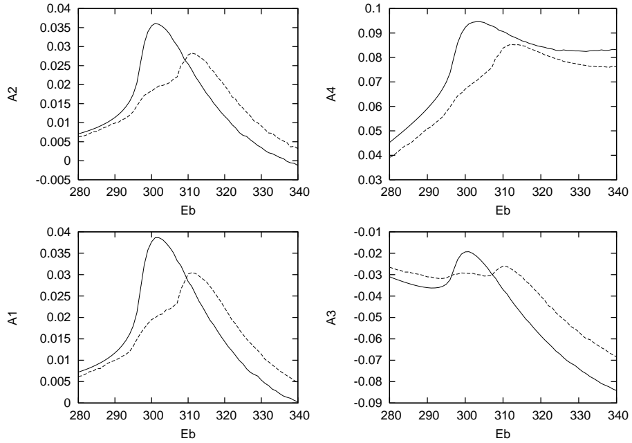
Figure 8: Four of the asymmetries of Eq. 9 for the ideal and for the realistic spectrum.
