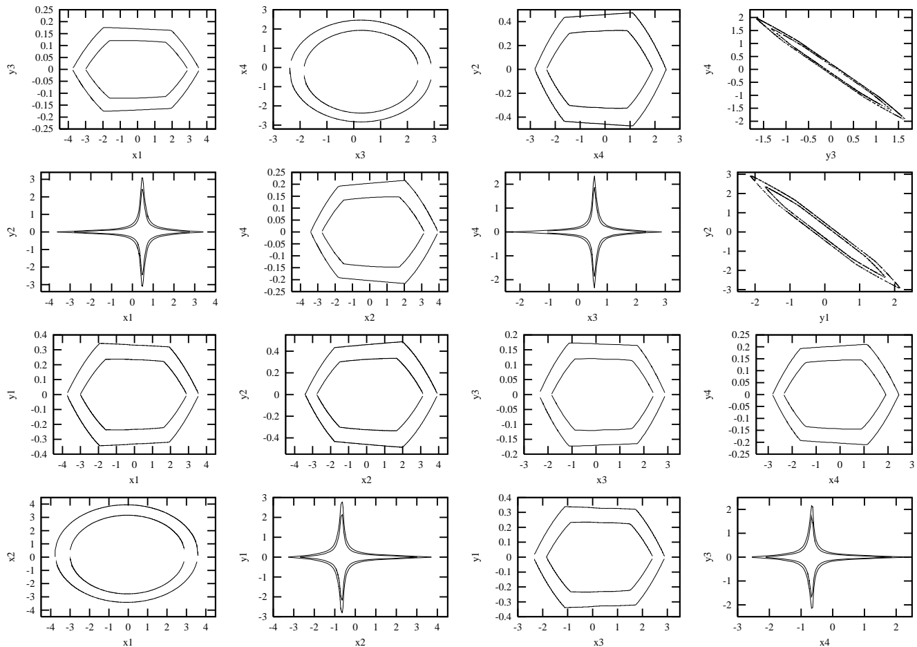
Figure 4: Blind regions in the various x_i - y_j planes, the larger and smaller region corresponding to luminosity 500\text{fb}^{-1} , 1000\text{fb}^{-1} respectively.
