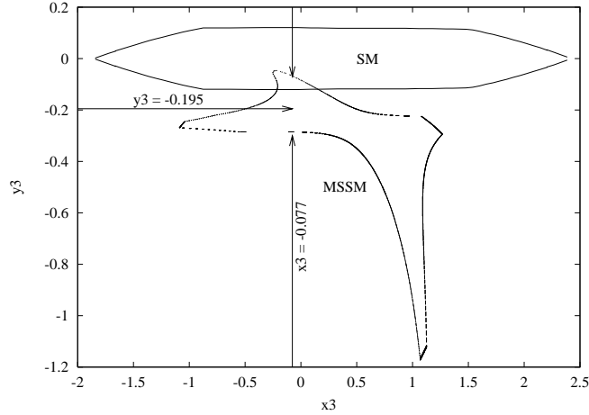
Figure 5: Blind regions for the chosen MSSM point and that for the plain SM QED contribution for 1000fb -1 at 95% CL.
