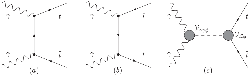
Figure 1: Feynman diagrams for the t\bar{t} production in \gamma\gamma collisions.
