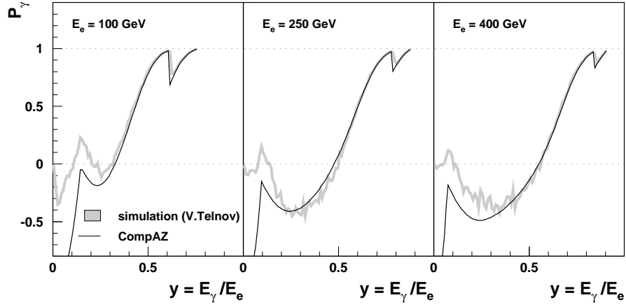
Figure 7: The polarisation P_\gamma for the backscattered laser photon as a function of the fraction of the beam energy carried by the photon, after inclusion of the nonlinear effects as parametrised in [12] and compared with simulation [13], for E_{beam} = 100, 250 and 400 GeV.
