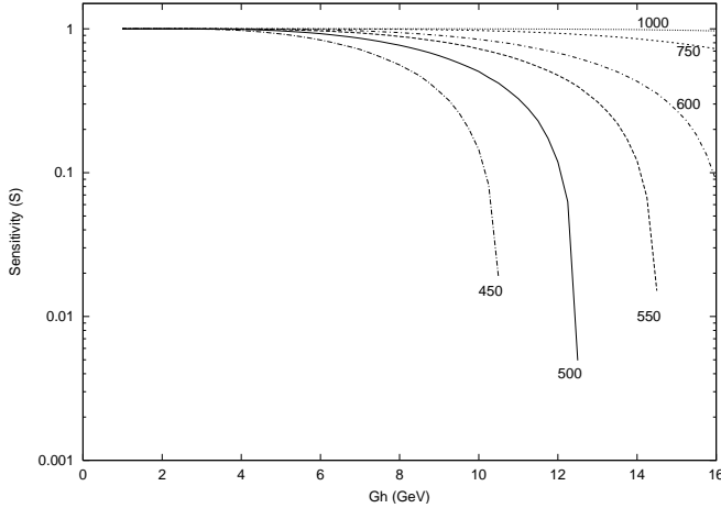
Figure 10: S_1 as a function of width of the scalar \Gamma_\phi for different luminosities for the chosen MSSM point and the ideal backscattered photon spectrum.
