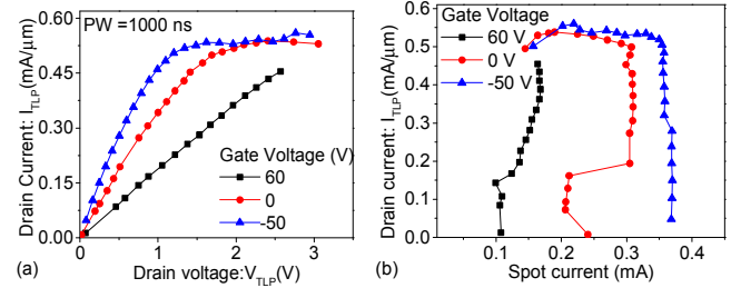
Fig. 6: (a) Pulse I-V characteristics of Graphene FET stressed with 1000 ns pulses to obtain the thermal SOA. Channel degradation at high gate-bias shrinks the thermal SOA. (b) The DC spot current data shows fall in drain current with increasing stress.
