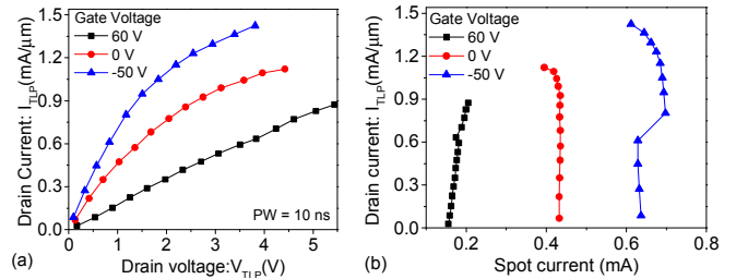
Fig. 5: Pulse I-V characteristics of GFET stressed with 10 ns wide pulses. Short duration pulse stressing mitigates thermal effects, and defines the near-electrical SOA. Near electrical failure thresholds are higher than the electro-thermal and thermal failure. (b) DC spot current measured after each pulse.
