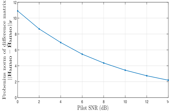
Fig. 5. Frobenius norm of the difference between the equivalent channel matrix ( \mathbf{H}_{\text{MIMO}} ) and the estimated equivalent channel matrix ( \hat{\mathbf{H}}_{\text{MIMO}} ) as a function of pilot SNR in a 2 \times 2 MIMO-OTFS system.
