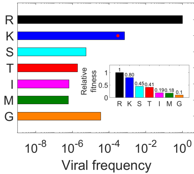
S1 Figure. Mutant spectrum at position 155 of NS3 using in vitro fitness estimates. Frequencies of the different mutants at steady state estimated as in Fig. 4 but using the fitness of different RAVs estimated in vitro (inset) [34]. Shown for comparison is the database value of the mutant R155K for HCV genotype 1a (red dot) [33].
