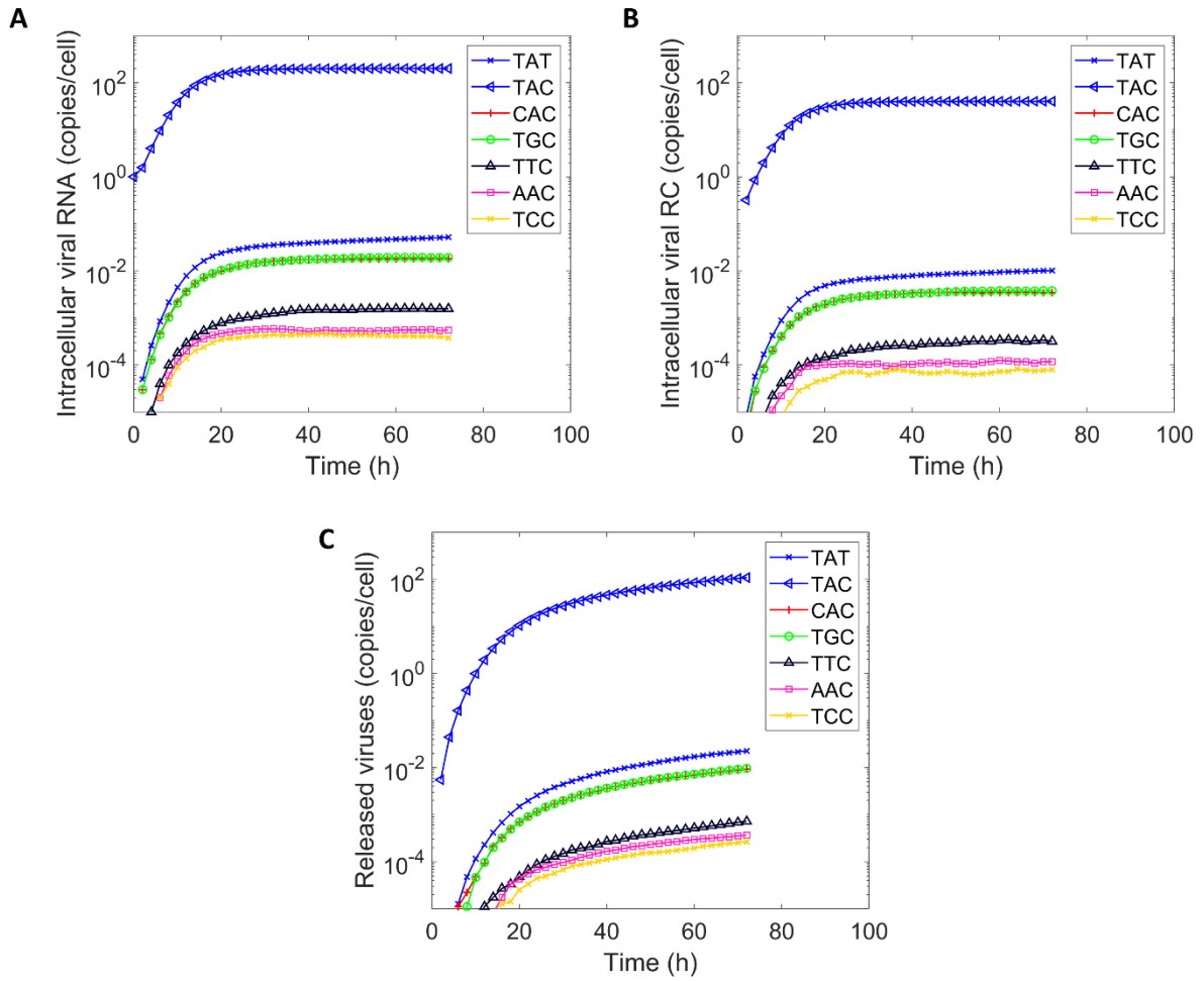
S6 Figure. Intracellular dynamics and evolution leading to NS5A resistance. The averaged evolution of the populations of genomes carrying different codons following infection with TAC at the position 93 of the NS5A region of HCV.
