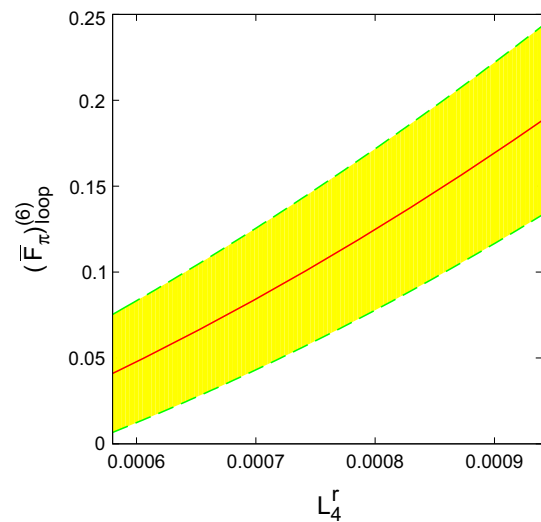
Fig. 2 L_4^r dependence of (\overline{F}_\pi^{(6)})_{\text{loop}} . The full line is the value for L_4^r = 0.49 \times 10^{-3} , while the shaded area indicates the range of possible values corresponding to the \pm 0.25 uncertainty of L_4^r in the free fit
