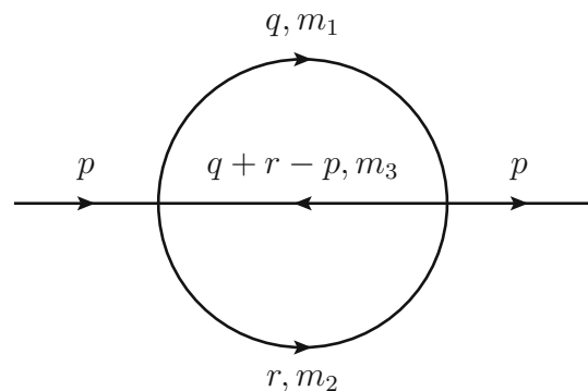
Fig. 1 The two-loop self-energy “sunset” diagram
