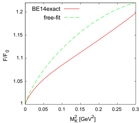
Fig. 4 M_K^2 dependence of F/F_0 in the chiral limit
