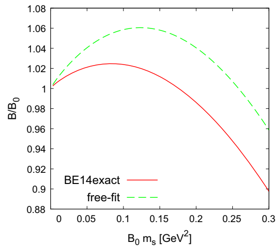
Fig. 5 m_s dependence of M_\pi^2/m_\pi^2 in the chiral limit
