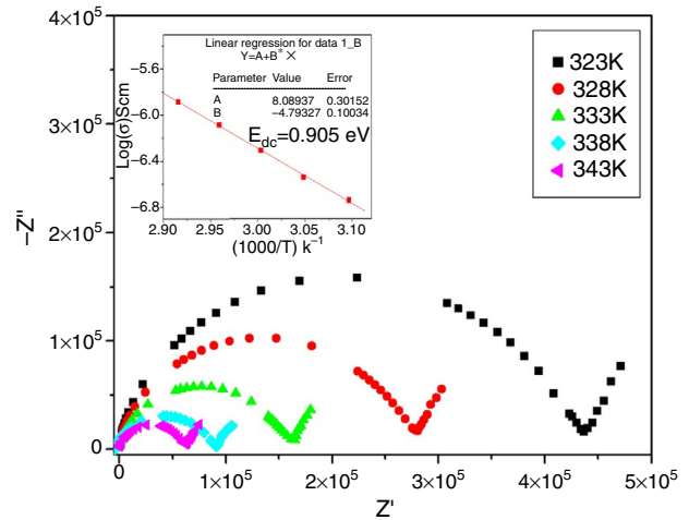
Fig. 5 – Impedance plot of VBZ 1 glass. Inset: Variation of \log(\sigma) versus 1000/T for VBZ 1 glass.
