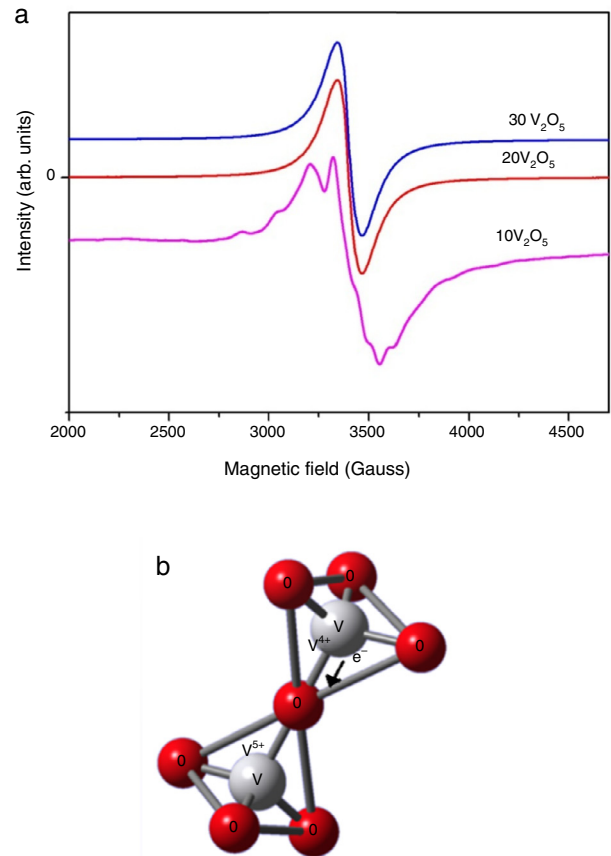
Fig. 7 – (a) EPR spectra of xV 2 O 5 ·20Li 2 O·(80 – x) [0.6B 2 O 3 ·0.4ZnO] glasses. (b) Schematic representation of electron hopping via V 4+ –O–V 5+ bonds.
