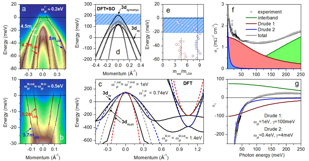
Figure 1. Low-energy electronic properties of \text{NaFe}_{0.978}\text{Co}_{0.022}\text{As} . (a,b) Low-energy electronic structure of \text{NaFe}_{0.978}\text{Co}_{0.022}\text{As} in the normal state near the \Gamma ((a) 30 K) and M ((b) 22 K) points of the Brillouin zone recorded using 20 eV and 25 eV photons linearly polarized perpendicular to and within the plane of incidence, respectively. The dispersion of all electronic bands observed in experiment (black solid lines) has been obtained using a multi-Lorentzian fit of the momentum-distribution curves. Effective-mass renormalization indicated in the panels has been calculated by comparing the low-energy parabolic fits to the electronic dispersions extracted from the experimental data (dashed lines in panels (a,b)) with those to the corresponding electronic bands predicted theoretically (dashed lines in panel (c)). (c) Theoretically predicted low-energy electronic band structure of \text{NaFeAs} in the \Gamma - M high-symmetry direction of the Brillouin zone (black solid lines) and low-energy parabolic fits to the dispersions near \Gamma and M (dashed lines). The colors of the dashed lines correspond to those in panels (a,b). Plasma frequencies of all bands crossing the Fermi level extracted from experimental data and predicted by theory are shown in panels (a–c). (d) Electronic band structure in the \Gamma - M high-symmetry direction of the Brillouin zone near the \Gamma point obtained in a relativistic DFT calculation (black lines), which explicitly accounts for a finite spin-orbit coupling (its characteristic energy scale is shown as blue hatched area). The results of the corresponding non-relativistic calculation from panel c are shown for comparison (grey lines). (e) Energy dependence of the effective mass renormalization in the outer (blue open circles), middle (grey circles), and inner (red circles) hole band at the \Gamma point with respect to the corresponding low-energy quasiparticle masses extracted from the theoretically predicted band structure in panel (c) using parabolic fits. The energy scale affected by spin-orbit interaction is indicated as a blue hatched area. (f,g) Real part of the optical conductivity (f) and the dielectric function (g) of \text{NaFe}_{0.978}\text{Co}_{0.022}\text{As} obtained in OS measurements (open circles) along with the results of a Drude-Lorentz dispersion analysis (blue and red lines/shaded areas and green line/shaded area for the two Drude terms and the total contribution of all interband transitions, respectively; gray solid lines indicate the sum of all terms). The parameters of the itinerant charge carrier response obtained by means of this analysis are summarized in panel (g).
