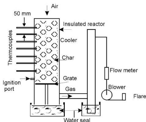
Figure 1. Experimental set-up for the packed-bed reactor.
