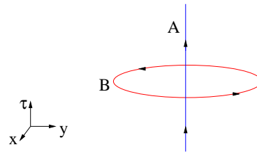
FIG. 1: Configuration with Q = 1 showing the location of the vortices in z_1 and z_2 . The curve A is the vortex in z_2 and B is the vortex in z_1 .
