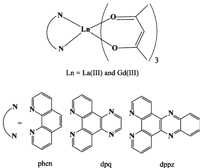
Figure 10. La(III) and Gd(III) complexes of phenanthroline bases and acetylacetonate ligand.
