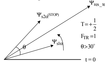
Fig.34.a. Phasor diagram.
