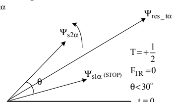
Fig.34.b. Phasor diagram
