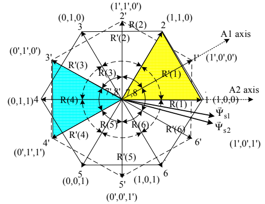
Fig.13. Sector identification
