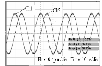
Fig.24.Ch1: \Psi_{res\alpha} Ch2: \Psi_{res\beta}
