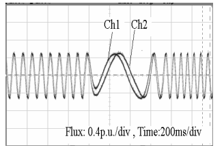
Fig.28. Fluxes during speed reversal Ch1: \Psi_{s\alpha 1} Ch2: \Psi_{s\alpha 2}
