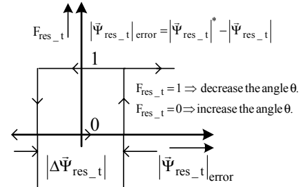
Fig.14. Angle Controller
