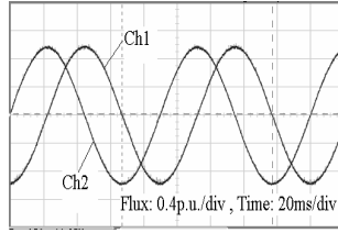
Fig.19.Ch1: \Psi_{res\beta} Ch2: \Psi_{res\alpha}
