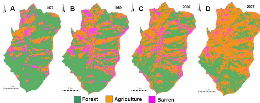
Figure 3. GMLC based LU classification using (A) Landsat MSS, 1972, (B) Landsat TM, 1989, (C) Landsat ETM, 2000 and (D) IRS LISS-III, 2007.
