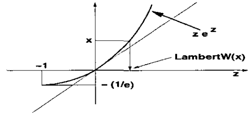
Fig. 9. The LambertW function is the inverse function of ze^z ; notice that for x \geq -1/e , LambertW(x) \leq x , with equality only for x = 0 .
