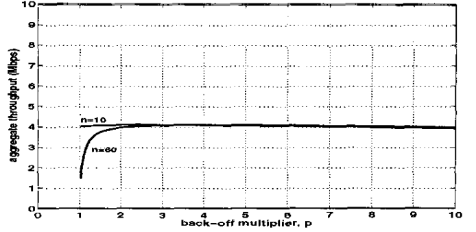
Fig. 10. Aggregate throughput plotted vs. the back-off multiplier p for two values values of n . The network parameters are K = 10 , b_0 = 16 slots, data packet length 8000 bits, packet overhead 592 bits, slot time 20 \mu s, transmission rate for all flows 11 Mbps, fixed (rate independent) data packet transmission overhead 52 slots, collision overhead 17 slots.
