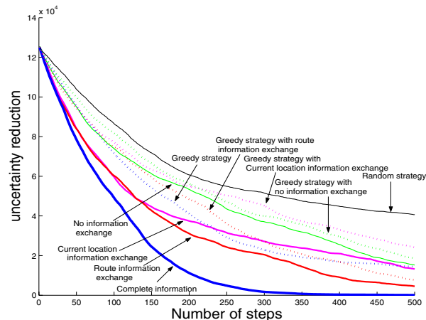
Fig. 7. Uncertainty reduction for large search space
