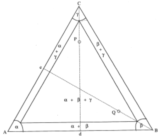
Figure 1. Isothermal section of the phase diagram at c = 3.5 (schematic).
