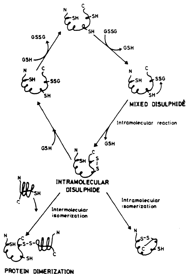
Figure 1. Fate of protein thiols and disulphides in the presence of oxidized (GSSG) and reduced (GSH) glutathione. Conformational change in the protein has been envisaged during intramolecular disulphide bond formation or intramolecular isomerization of disulphide bond.
