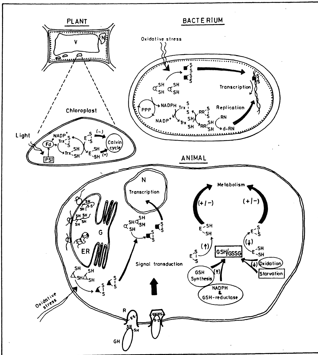
Figure 2. A diagrammatic representation of cellular events controlled by thiol/disulphide exchange reaction. Key: V, vacuole; N, nucleus; ER, endoplasmic reticulum; G, golgi; E, enzyme; GH, gonadotropin hormone; Fd, ferredoxin; PSI, photosystem I; R, receptor; RR, ribonucleotide reductase; RN & d-RN, ribo- and deoxy-ribonucleotides; Trx, thioredoxin; α-SH, inactive transcriptional activator; α-S-S, active transcriptional activator; α-SH, redox-active transducer protein.
