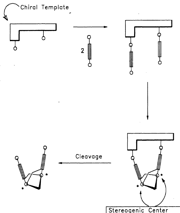
Figure 9. Schematic representation of coupling on a template.
