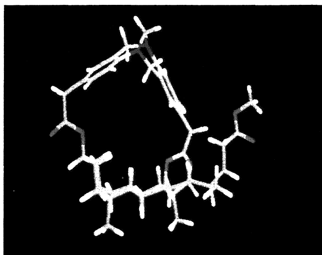
Figure 8. DTMM modelled structure for the Tröger's base unit (S,S at N) on the steroid template.
