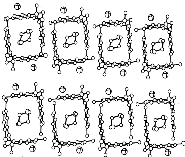
Figure 5. Perspective view of the molecular packing in 12b (dioxane) 0.5 clathrate. H atoms are not shown. Dioxane molecules are embedded in the void formed by the pairs of quaternary Tröger's base units. Reproduced with permission of the Royal Society of Chemistry.
