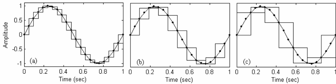
Fig. 2. Multiresolution box-counting approach for sinusoidal signal, (a) at the finest time resolution, and (b) and (c) at the next two coarse time resolution.
