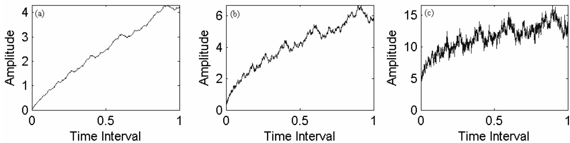
Fig. 5. Weierstrass-Mandelbrot cosine function, N = 1025 , b = 1.5 , M = 100 , (a) D = 1.2 , (b) D = 1.5 , (c) D = 1.8 .
