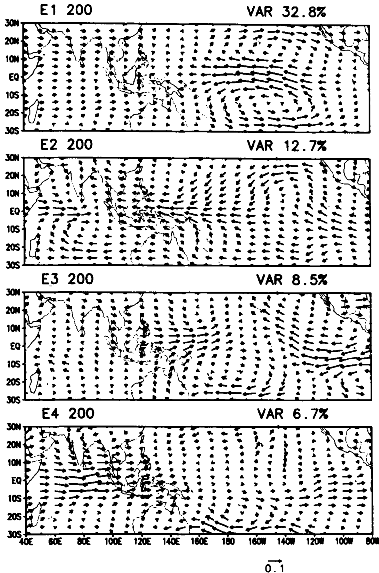
Figure 4. Same as figure 3 but for 200 mb.
