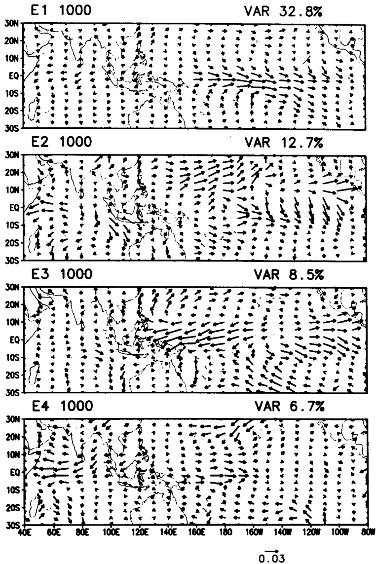
Figure 3. First four vector EOFs of the winds at 1000 mb. The combined per cent variance explained is also given.
