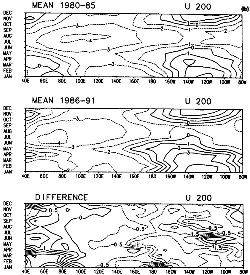
Figure 10(a and b). Annual cycle of climatological zonal wind averaged over 5°S–5°N for the two periods and the difference between these two climatologies at (a) 850 mb and (b) 200 mb.
