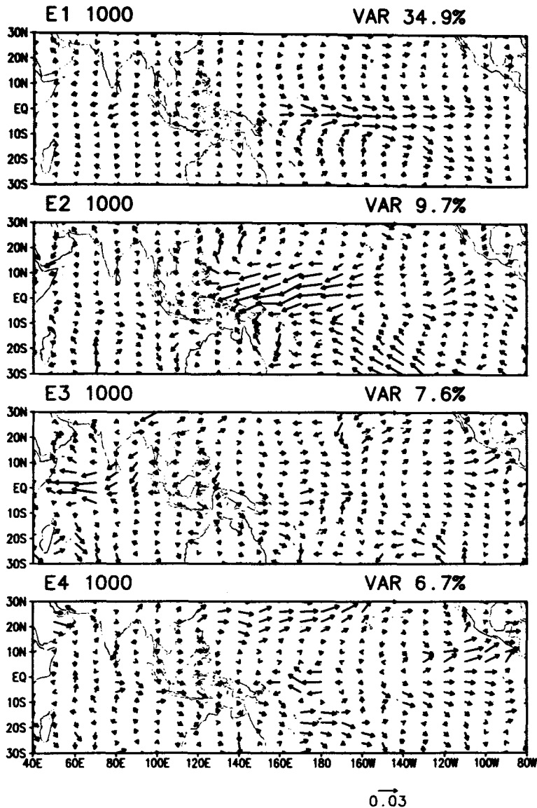
Figure 12. Same as figure 3 but for the anomalies formed with respect to the two climatologies.
