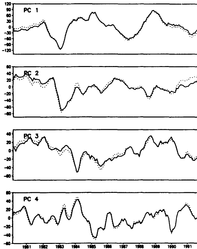
Figure 11. The first four PCs of the combined EOFs of zonal and meridional winds at 1000, 850 and 200mb but for anomalies formed from the detrended analysis (solid curve) and anomalies formed with respect to the two climatologies (dashed line).
