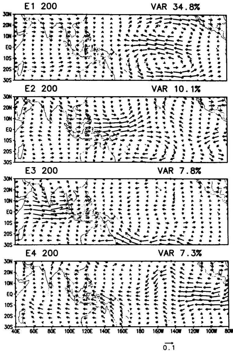
Figure 9. Same as figure 8 but for 200 mb.
