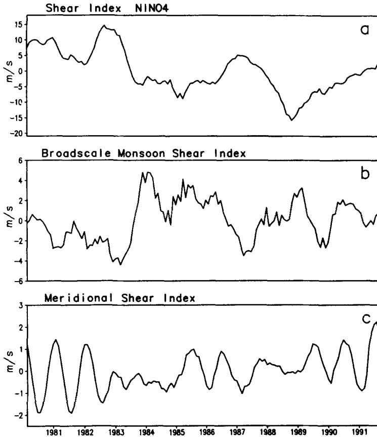
Figure 1. Anomaly time series, based on the 1980–1991 data. (a) The shear index, ( U_{850} - U_{200} ) averaged over the NINO-4 ( 5^{\circ}\text{S} - 5^{\circ}\text{N} , 160^{\circ}\text{E} - 150^{\circ}\text{W} ) region of the Pacific; (b) Broadscale monsoon index ( U_{850} - U_{200} ) averaged between 40^{\circ}\text{E} - 110^{\circ}\text{E} and 5^{\circ}\text{N} - 20^{\circ}\text{N} ; (c) The meridional shear index, ( V_{850} - V_{200} ) averaged over the equatorial Indian Ocean ( 10^{\circ}\text{S} - 10^{\circ}\text{N} , 40^{\circ}\text{E} - 110^{\circ}\text{E} ).
