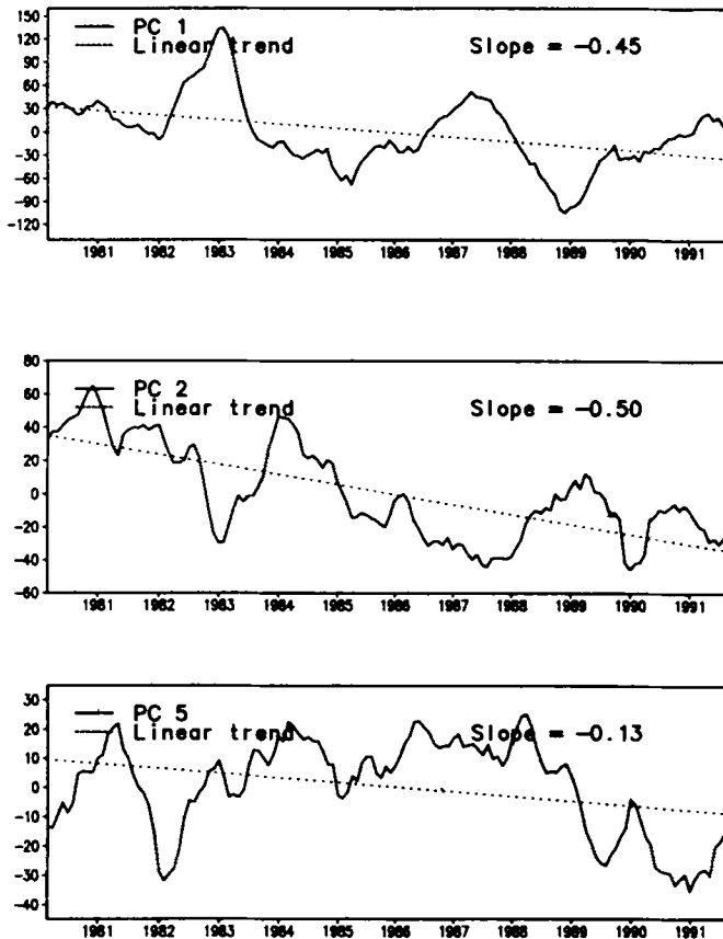
Figure 7. The linear trends obtained for the dominant PCs of figure 2. Shown also is the slope obtained from least squares fit.
