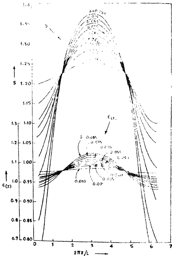
FIG. 2 b . \epsilon_s and spacing vs 2\pi z/L for case 4. \epsilon^0 = 1.062 , b = 0.6 cm, S = 1.5 cm, a = 0.25 cm.
