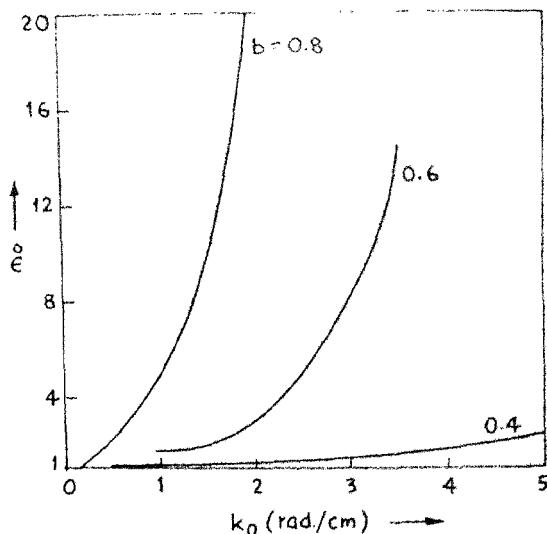
FIG. 1 g. Variation of \epsilon^0 with k_0 for S = 0.2 cm, b as parameter.
