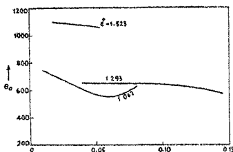
FIG. 6 (a). Variation of \theta_0 with \delta , with \epsilon^0 as parameter.
