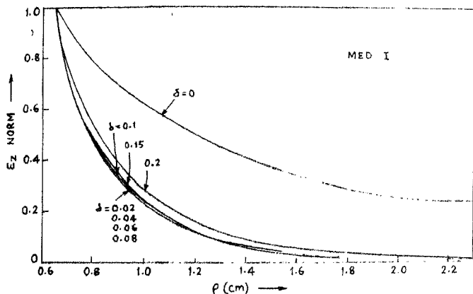
a. 8 (b). E_z vs \rho for \epsilon^a = 1.293 in medium I.
