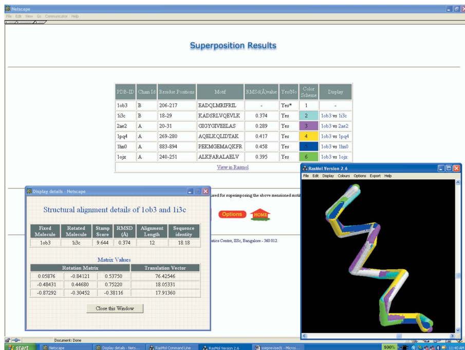
Figure 2 An output frame showing the detailed superposition results output for five \alpha -helical segments of 12 residues (exact length) as queried by the search engine from 90% non-redundant protein chains.
