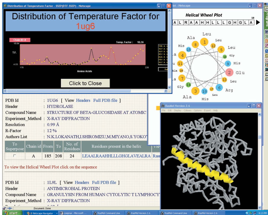
Figure 1 A screen shot of the output frame displaying some of the structural properties of an \alpha -helix with 24 residues present in a \beta -glucosidase (resolution, 0.99 Å; crystallographic R factor, 12%).
