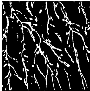
(g) 140s membrane in 15 cm \times 15 cm tank, Ra = 5.36 \times 10^{11} , \Delta C = 8.42 g/l, Q = 0.41 mg/cm ^2 /min, W_* = 0.48 cm/s, Re = 1236.3 , V_I = 0.0016 cm/s, Image area = 7.58 cm square, 616^2 pix
