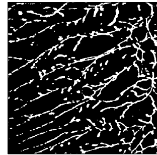
(f) 140s membrane in 15 cm \times 15 cm tank, Ra = 4.49 \times 10^{11} , \Delta C = 7.06 g/l, Q = 0.41 mg/cm ^2 /min, W_* = 0.48 cm/s, Re = 1236.3 , V_I = 0.0023 cm/s, Image area = 8.32 cm square, 520^2 pix
