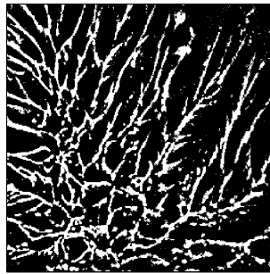
(e) 140s membrane in 15 cm \times 15 cm tank, Ra = 5 \times 10^{11} , \Delta C = 7.87 g/l, Q = 0.39 mg/cm ^2 /min, W_* = 0.47 cm/s, Re = 1210.5 , V_I = 0.002 cm/s, Image area = 8.61 cm square, 528^2 pix
