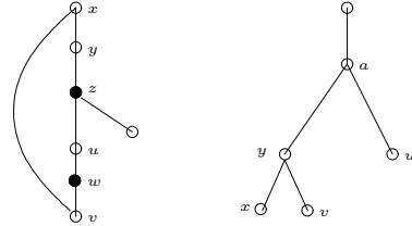
Figure 1: The Contiguity Problem: Trees T_1 and T_2
