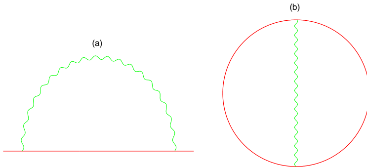
Figure 1: Typical divergent diagrams quadratic in the spurion sources (a) with an open quark line (b) with a closed quark line.
