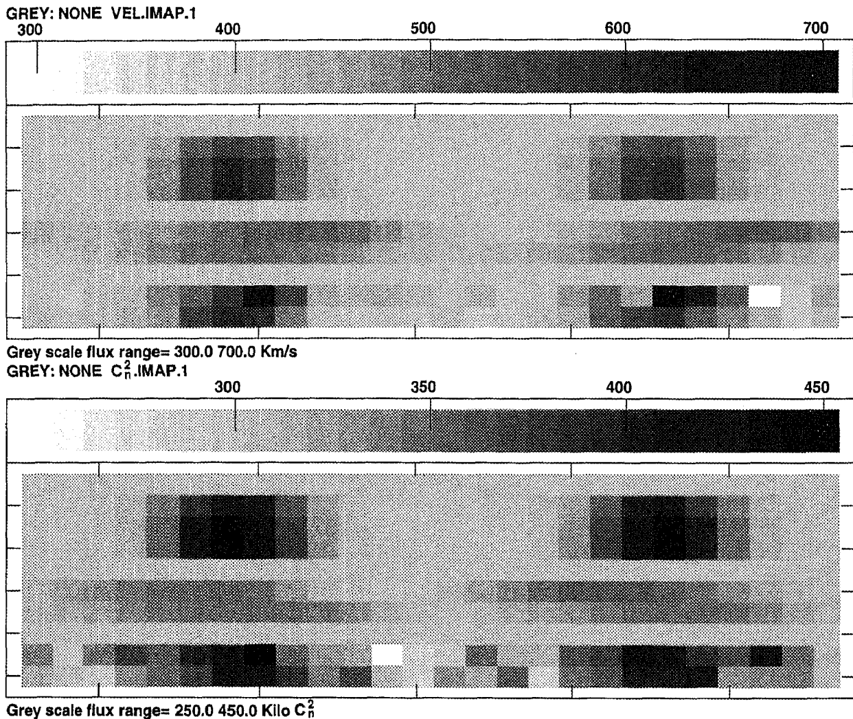
Figure 1. Velocity and C_n^2 maps - In the top figure, the first panel shows the input model which was used to simulate the IPS data, the second panel the initial guess which was computed from the simulated data and was used as input for the reconstruction procedure and the third panel shows the final reconstructed model for velocity of the SW. The bottom figure shows the same set of plots for C_n^2 (in arbitrary units). The first panel shows a heliographic range of [+10^\circ, -20^\circ] and the second and the third panels that of [+12^\circ, -20^\circ] . The pixel size in the reconstructed surface distribution is 13.3^\circ in longitude and 16^\circ in latitude.
